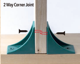
2 Way Corner Joint
