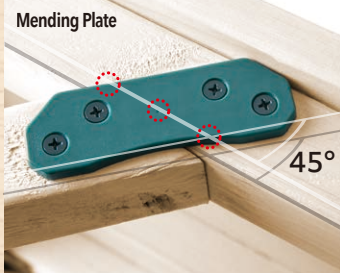
Mending Plate
